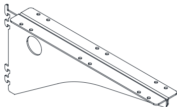
Standard Panel Mounted Cantilever Arm
