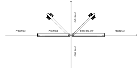
4-Way Connection, 2 Doors
