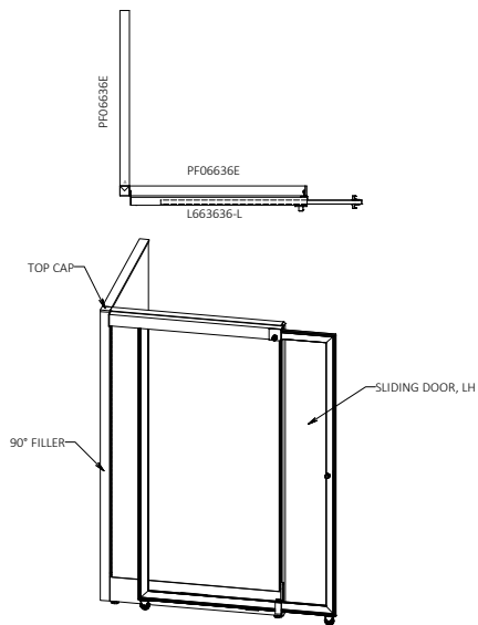
2-Way 90° Connection
